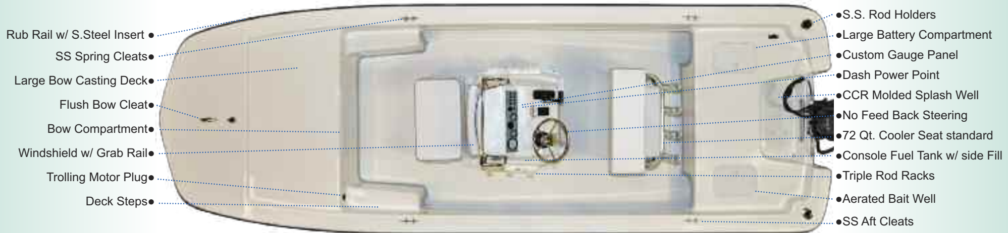
Shown Below With standard FB Console and Optional Leaning Post and Cooler in Front of console
