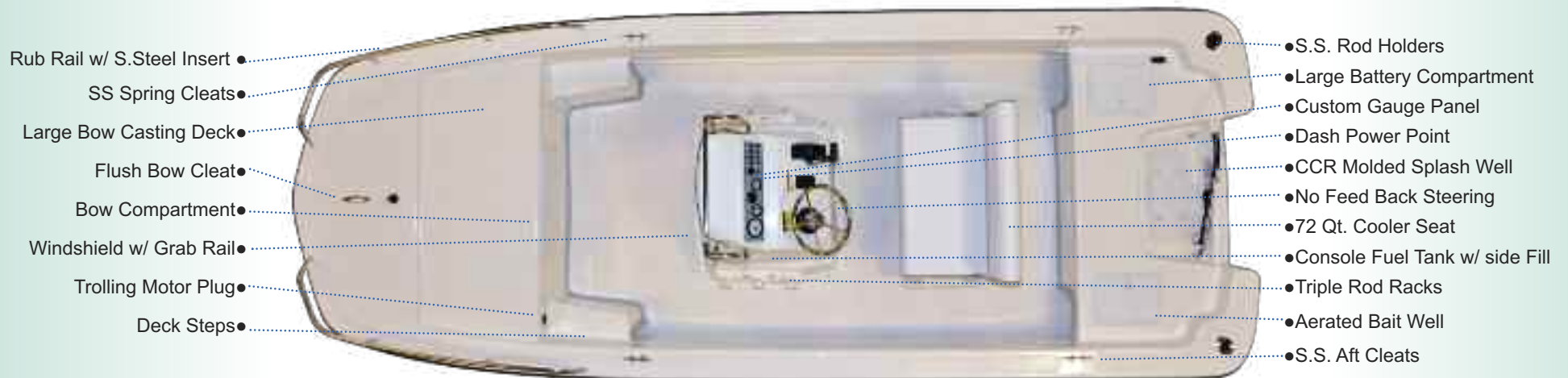
Shown Below with Standard FB Console and Flip Cooler Seat and Optional Bow Rails
